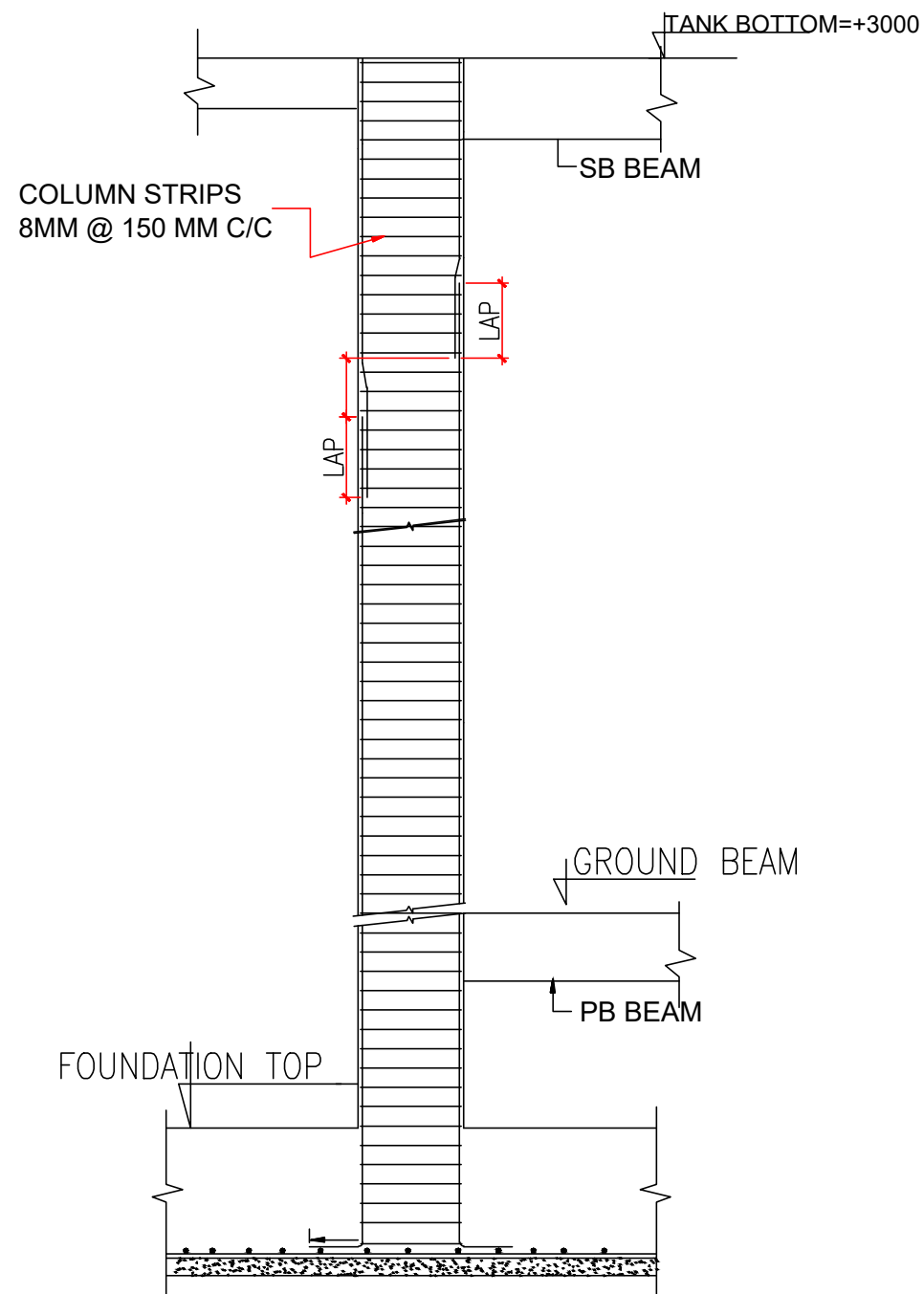
DET. OF COLUMN REINFORCEMENT
