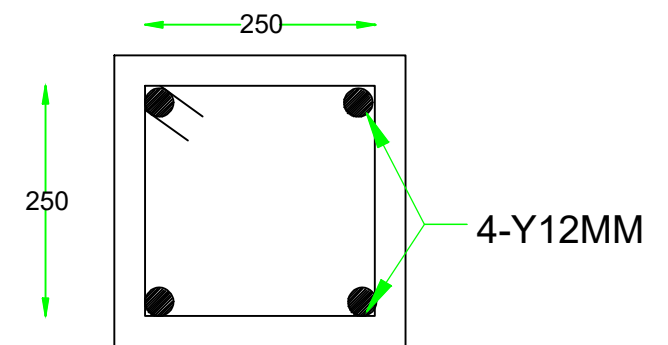
Slab Beam
