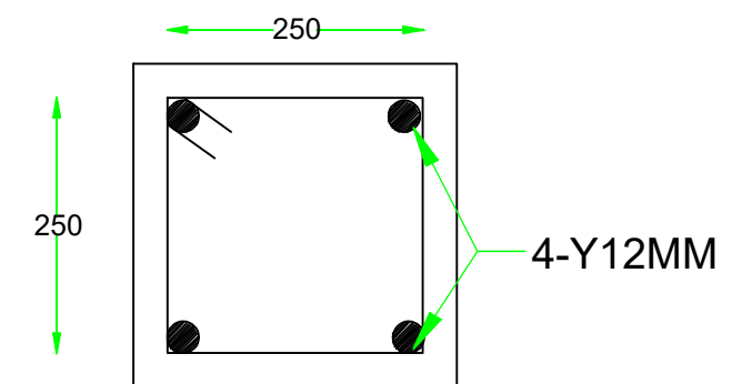
CROSS SECTION PB & SB
