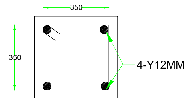
COLUMN
