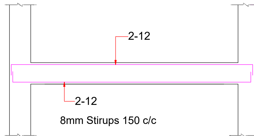
CROSS SECTION SB
